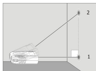
Indirect height measurement (Pythagorean)
